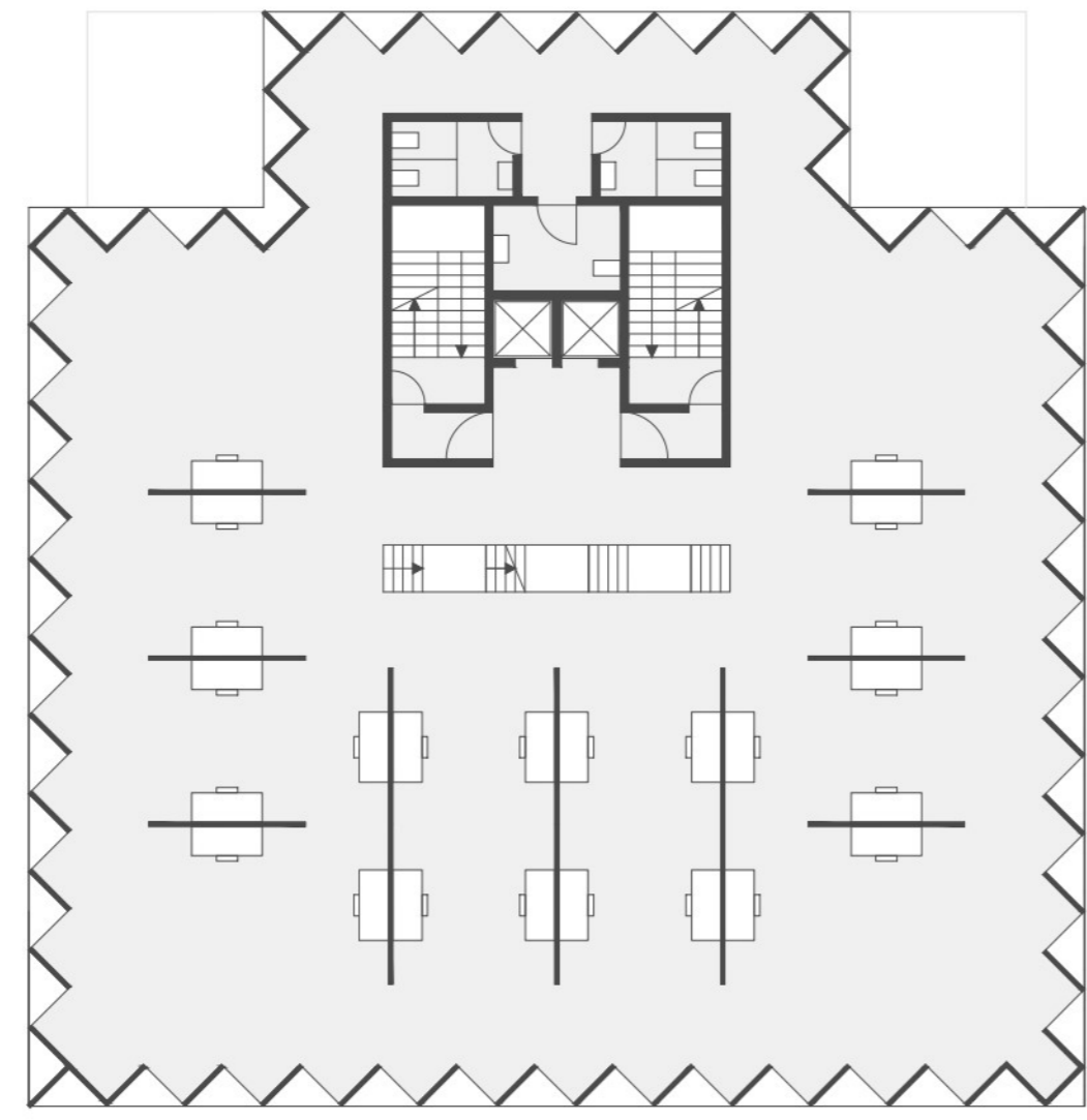
piso 4 | open space
