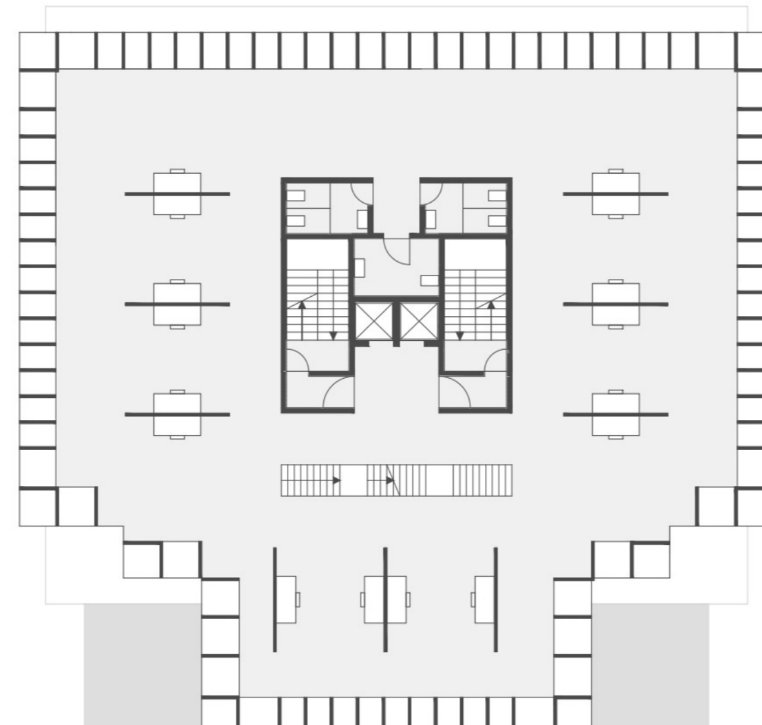
piso 9 | open space
