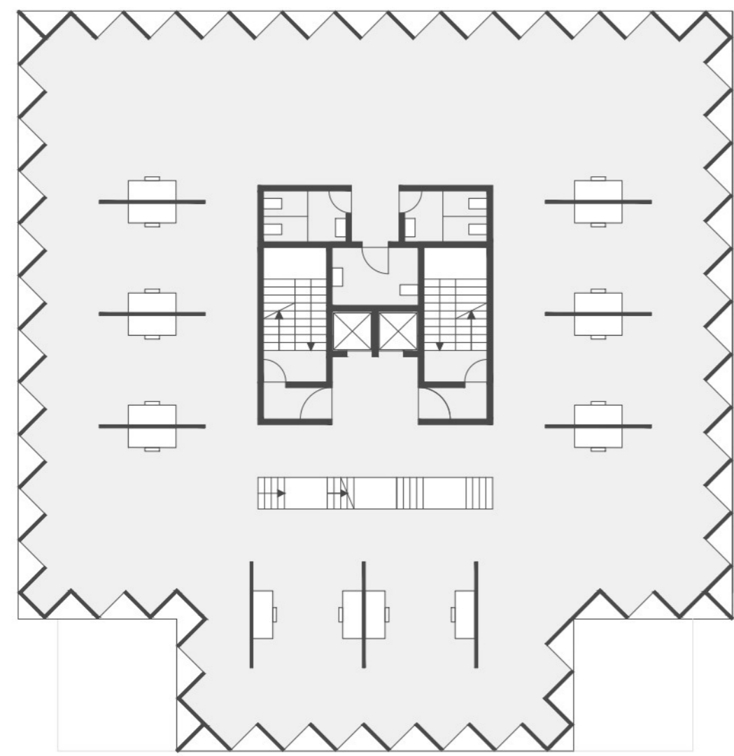
piso 8 | open space
